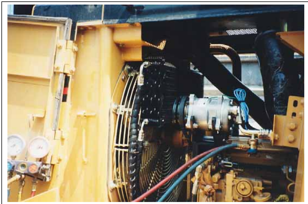
Right side of condenser mounted to fan screen
