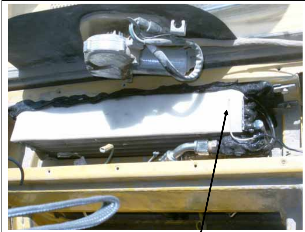
Thermostat probe location under foam
